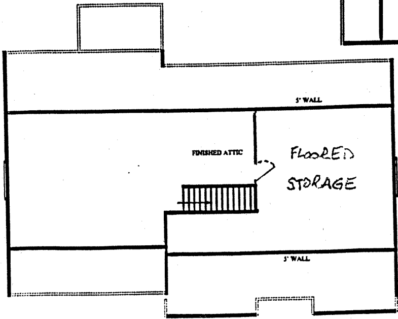
ATTIC PLAN
