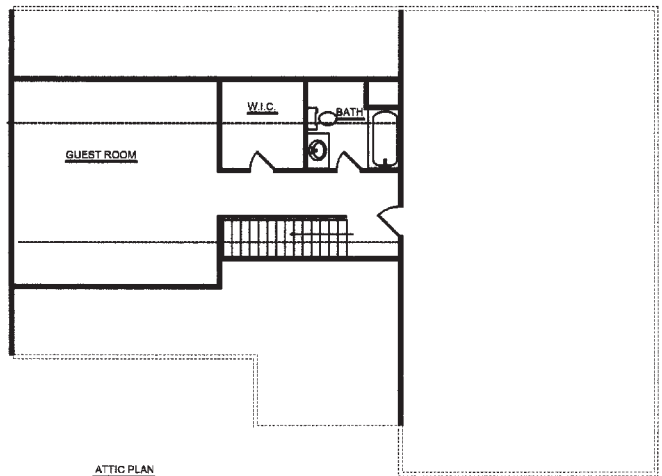
ATTIC PLAN
